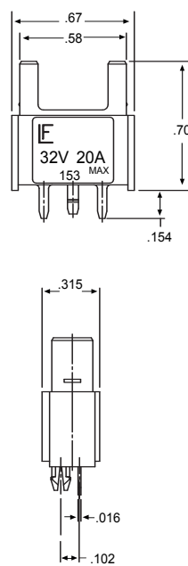
Single or stackable end unit (Part No. 01530032)
