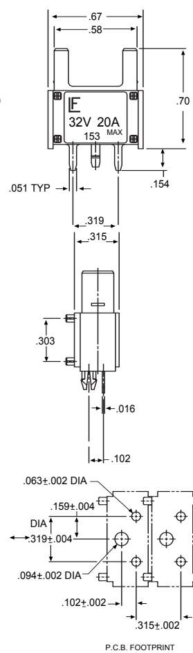
Stackable unit (Part No. 01530033)
