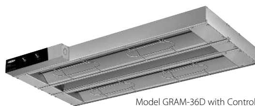
Model GRAM-36D with Control box (includes toggles) and 3" (76 mm) spacer
