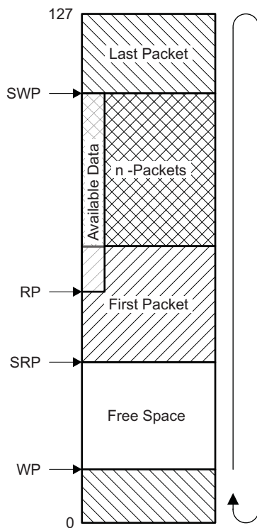
Figure 25-2. FIFO Pointers
